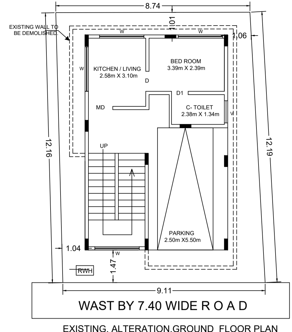
EXISTING ALTERATION GROUND FLOOR PLAN
